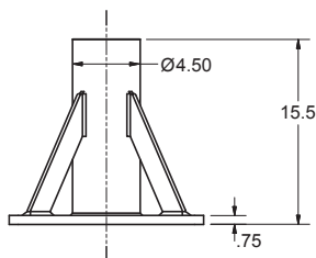
Pedestal base
