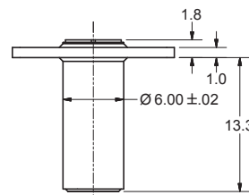
Socket base
